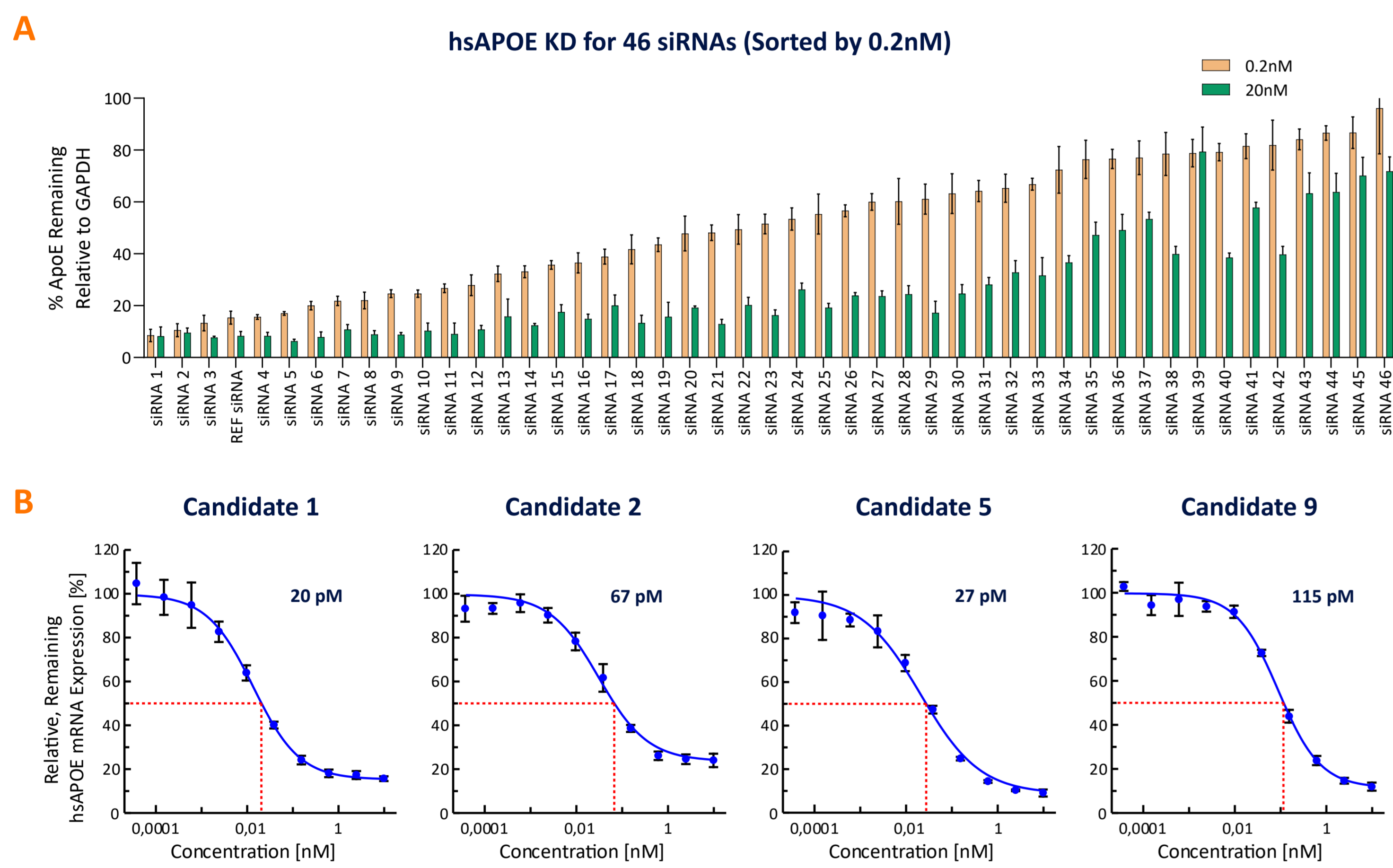
Figure 1. In vitro siRNA Screening Identifies Multiple Potent APOE-targeting siRNAs
