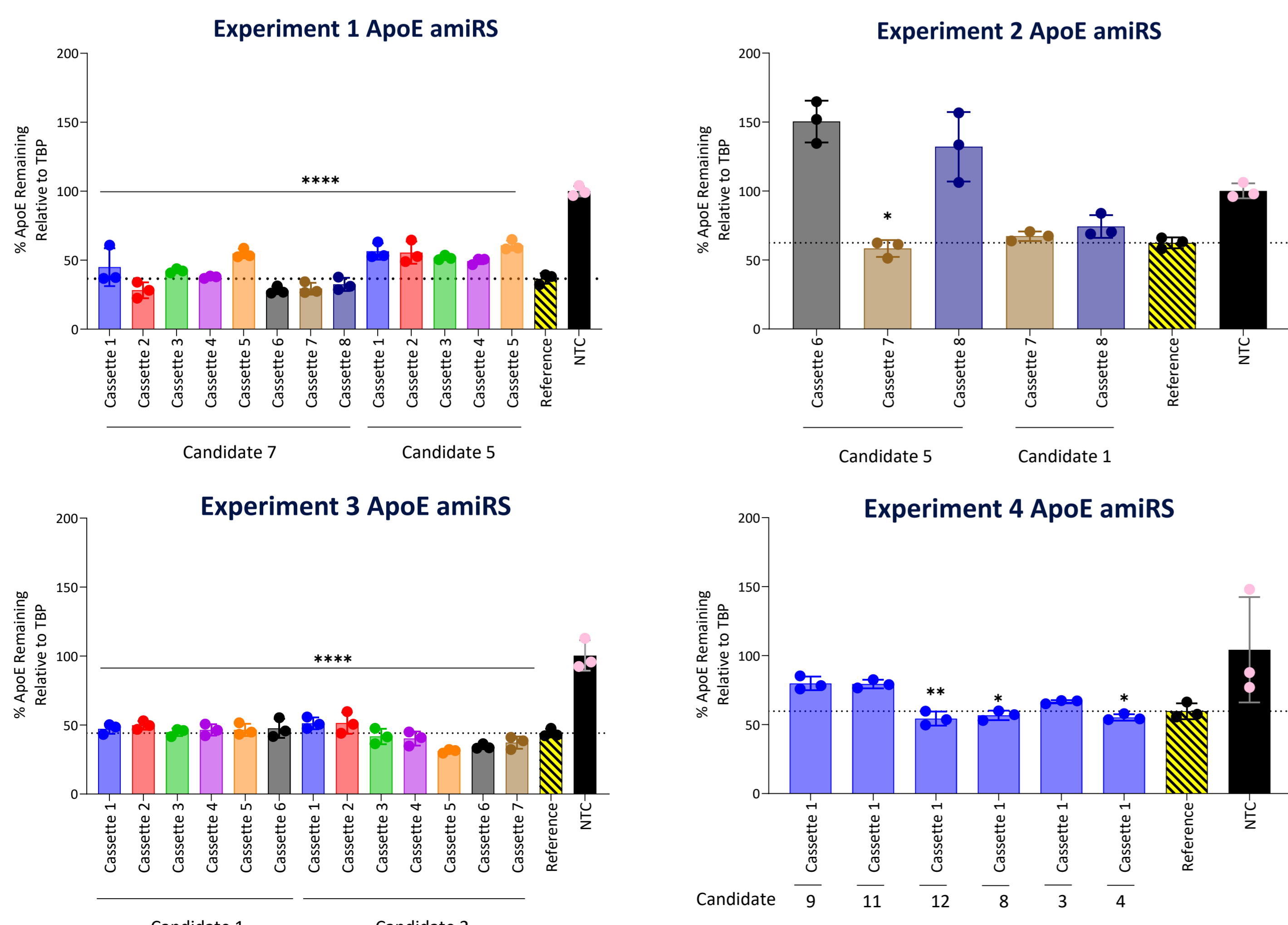
Figure 2. Projected Therapeutic Level of hAPOE Silencing Achieved with amiRNAs in vitro
