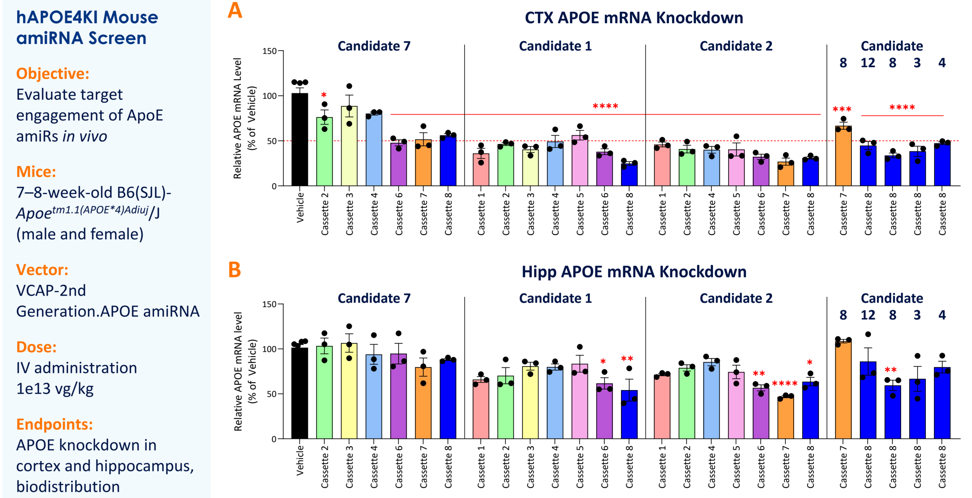
Figure 3. Single IV-dose Delivery of APOE miRNA via VCAP Gen. 2 Capsids Results in Robust APOE mRNA Reduction in Key AD Brain Regions
