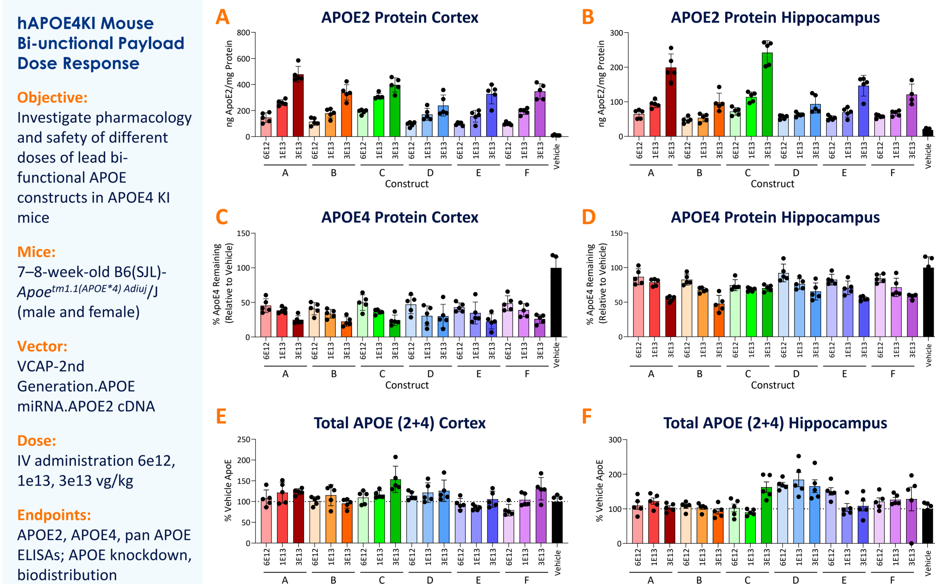
Figure 4. A Single IV Injection of Bi-functional Vector Leads to a Dose Dependent hAPOE4 Protein Reduction and hAPOE2 Delivery in Mouse Cortex and Hippocampus
