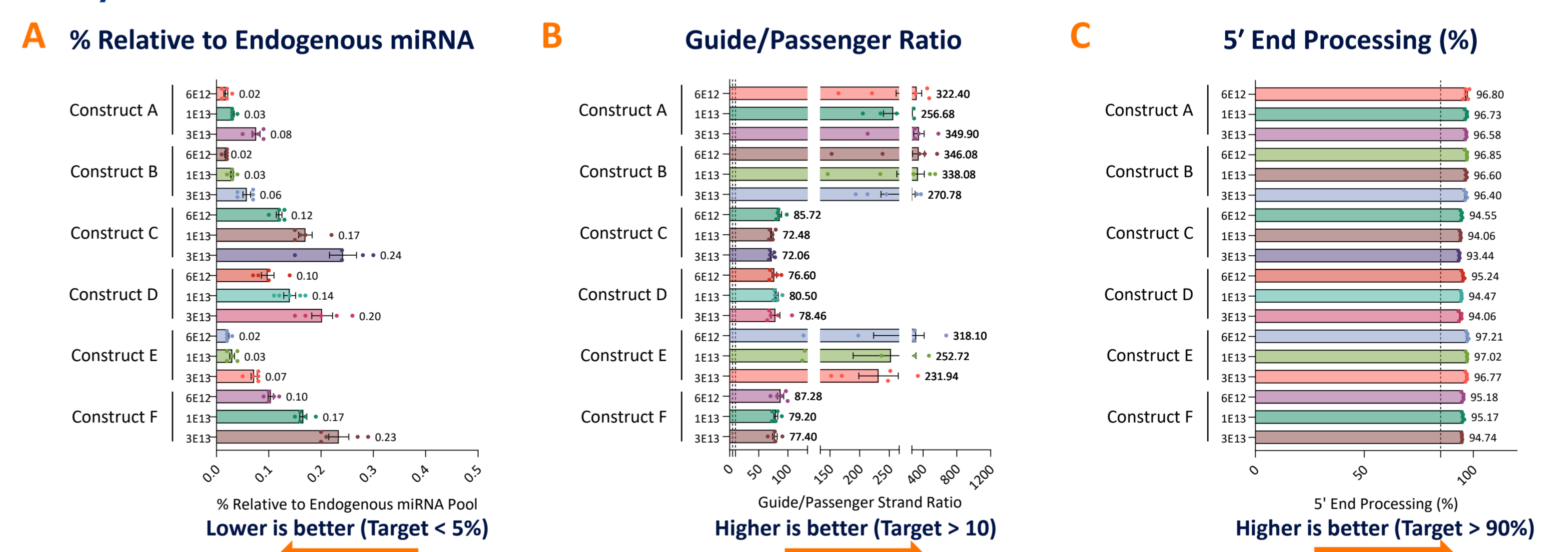
Figure 5. Global miRNA Profiling Identifies Several Candidates with Favorable amiR Safety Profile
